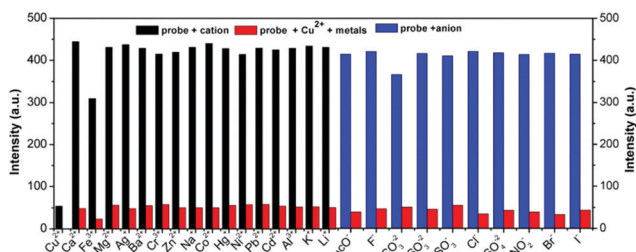
Fig. 5 Bar diagram of the competitive experiments of various metal cations and anions on the fluorescence intensity of the probe/ \text{Cu}^{2+} complex in buffer solution ( \lambda_{\text{ex}}/\lambda_{\text{em}} = 415/598 \text{ nm} , slit: 5/5 nm, voltage: 900 V).
