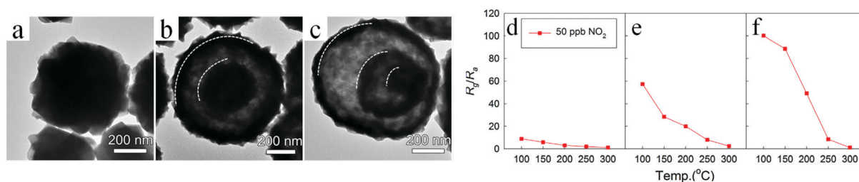
Fig. 43 TEM images of (a) D- \text{WO}_3 , (b) 2S- \text{WO}_3 , and (c) 3S- \text{WO}_3 . Gas responses ( R_g/R_a ) to 50 ppb \text{NO}_2 of (d) D- \text{WO}_3 spheres, (e) 2S- \text{WO}_3 spheres, and (f) 3S- \text{WO}_3 spheres. Reprinted from ref. 223 with kind permission.
