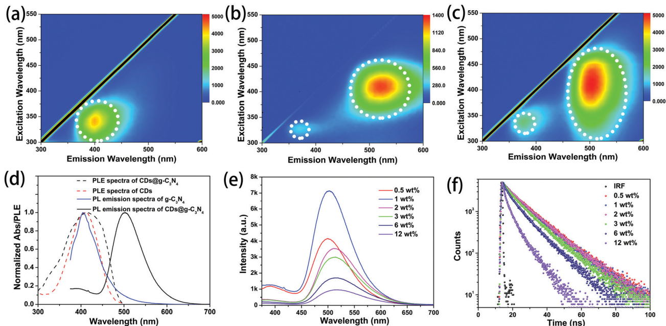
Fig. 4 Excitation–emission maps of (a) g\text{-C}_3\text{N}_4 solid powder, (b) an ethanolic solution of CDs and (c) a solid powder of a \text{CDs@g-C}_3\text{N}_4 composite with 1 wt% CDs. (d) PLE spectra (monitored at 510 nm) of CDs (red dotted curve) and \text{CDs@g-C}_3\text{N}_4 (black dotted curve), and PL emission spectra (excited at 360 nm) of g\text{-C}_3\text{N}_4 (blue curve) and \text{CDs@g-C}_3\text{N}_4 (black curve). (e) PL spectra of \text{CDs@g-C}_3\text{N}_4 composites with different loadings of CDs, all excited at 360 nm. (f) PL decay curves of g\text{-C}_3\text{N}_4 and \text{CDs@g-C}_3\text{N}_4 powders with different loadings of CDs, monitored at 510 nm under 375 nm excitation.
