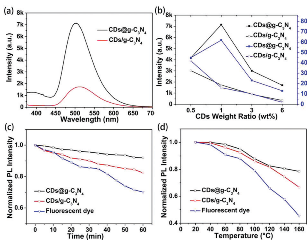
Fig. 5 (a) PL spectra of \text{CDs@g-C}_3\text{N}_4 and \text{CDs/g-C}_3\text{N}_4 composites with 1 wt% CD loading concentration under 360 nm excitation. (b) Peak PL intensities under 360 nm excitation of \text{CDs@g-C}_3\text{N}_4 and \text{CDs/g-C}_3\text{N}_4 with different CD loading concentrations (black curves) and PLQYs of \text{CDs@g-C}_3\text{N}_4 and \text{CDs/g-C}_3\text{N}_4 composites with different CD loading concentrations under 410 nm excitation (blue curves). Evolution of the PL intensities of \text{CDs@g-C}_3\text{N}_4 , \text{CDs/g-C}_3\text{N}_4 and organic dye (fluorescein sodium): (c) under UV light exposure ( 1.6\text{ W cm}^{-1} ) and (d) upon heating to 160\text{ }^\circ\text{C} .
