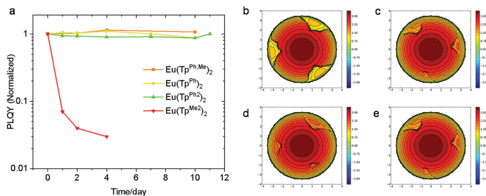
Fig. 3 (a) The normalized PLQY changes of crystalline Eu(Tp Me 2 ) 2 , Eu(Tp Ph,Me ) 2 , Eu(Tp Ph ) 2 and Eu(Tp Ph 2 ) 2 in air. Topographic steric maps of Eu(Tp Me 2 ) 2 (b), Eu(Tp Ph,Me ) 2 (c), Eu(Tp Ph ) 2 (d) and Eu(Tp Ph 2 ) 2 (e). Red and blue indicate the more- and less-hindered zones, respectively. 29
