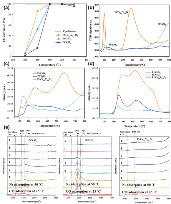
Fig. 15 (a) CO conversion of Pt/Y 2 O 3 , Pt/CeO 2 and Pt/Ce 0.6 Y 0.4 O 2 in the WGSR. (b) H 2 -TPR profiles of Pt/Y 2 O 3 , Pt/CeO 2 and Pt/Ce 0.6 Y 0.4 O 2 . (c) CO-TPR profiles of Pt/Y 2 O 3 , Pt/CeO 2 and Pt/Ce 0.6 Y 0.4 O 2 . (d) H 2 profile. (e) DRIFTS spectra of Pt/Y 2 O 3 , Pt/CeO 2 and Pt/Ce 0.6 Y 0.4 O 2 . (f) N 2 adsorption at 100 °C; (g) N 2 adsorption at 150 °C; (h) N 2 adsorption at 200 °C; (i) N 2 adsorption at 250 °C; (j) N 2 adsorption at 300 °C; and (k) N 2 adsorption at 350 °C. Adapted with permission from ref. 86. Copyright 2018, American Chemical Society.
