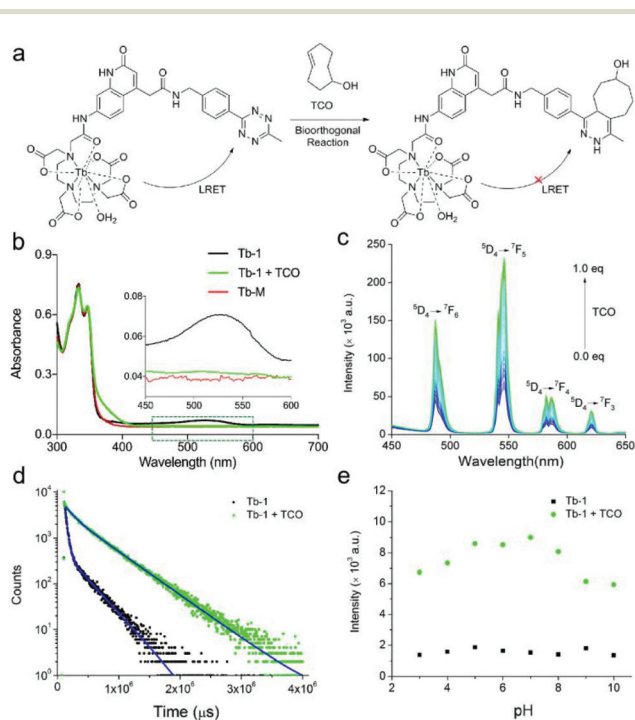
Fig. 2 (a) Schematic of sensing bioorthogonal reaction of luminogenic Tb-1 with TCO based on the LRET mechanism. (b) The absorbance spectra of Tb-M , and Tb-1 in the absence or presence of TCO. (c) Time-gated luminescence spectra of Tb-1 titrating with TCO ( \lambda_{\text{ex}} = 340\text{ nm} ). (d) Decay time curves of the ^5\text{D}_4 \rightarrow ^7\text{F}_5 emission of \text{Tb}^{3+} (10 \mu\text{M} ) in the absence and presence of TCO (20 \mu\text{M} ). (e) The luminescence intensity ( \lambda_{\text{em}} = 545\text{ nm} ) of complex Tb-1 reacted with TCO in various pH buffers.
