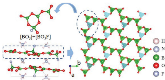
Fig. 3 Crystal structural features of \text{NH}_4\text{B}_4\text{O}_6\text{F} , whose FBU is composed of [\text{BO}_3] and [\text{BO}_3\text{F}] .
