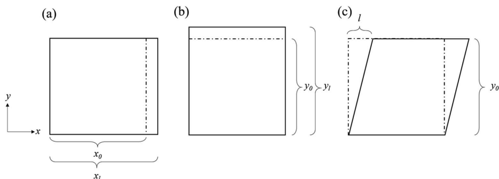
Fig. 2 The structures before strain (dashed line) and after strain (solid line). (a and b) BNNS under uniaxial strain \varepsilon_1 and \varepsilon_2 respectively. (c) BNNS under shear strain \varepsilon_6 .
