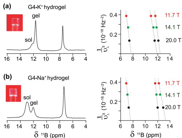
Fig. 2 Gel-state 1D ^{11}\text{B} MAS (5 kHz) NMR spectra of 20 \mu\text{L} G4-M ^{+} hydrogels acquired at 20 T using ^1\text{H} decoupling. The experimental ^{11}\text{B} NMR shifts of (a) G4-K ^{+} and (b) G4-Na ^{+} gels obtained at different magnetic fields are plotted as a function of the inverse squared Larmor frequency ( \nu_L^{-2} ) for both the GB mono (6–8 ppm) and diester signals (11–14 ppm). Sol and gel ^{11}\text{B} signals refer to borate mono- and diesters in a solution-like environment and in a G4 network, respectively.
