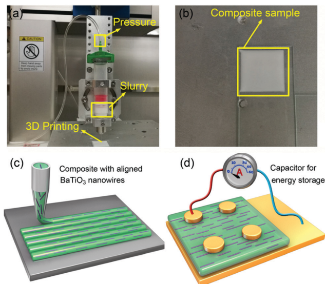
Fig. 1 Alignment of \text{BaTiO}_3 nanowires in nanocomposites: photographs of (a) the printing assembly and (b) a printed nanocomposite sample; schematic illustrations of (c) the alignment of \text{BaTiO}_3 nanowires in the P(VDF-CTFE) matrix and (d) a nanocomposite capacitor for energy storage applications.
