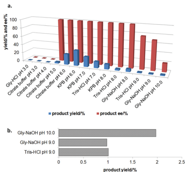
Fig. 1 (a) The pH effect on the activity of Oxd B in the catalytic asymmetric ring-opening of 5-phenyl-4,5-dihydroisoxazole. The reactions were performed on a 500 \mu L scale using 100 mM buffer (pH 3.0–10.0), 1 U Oxd-B, 20 mM 5-phenyl-4,5-dihydroisoxazole, 0.05 mM FMN, and 1 mM \text{Na}_2\text{S}_2\text{O}_5 at 30 ^\circ\text{C} for 30 min. The buffer solutions used were Gly-HCl (pH 3.0), Citrate-buffer (pH 3.0, 4.0, 5.0, and 6.0), KPB (pH 6.0, 7.0, and 8.0), Tris-HCl (pH 7.0, 8.0, and 9.0), and Gly-NaOH (pH 8.0, 9.0, and 10.0). (b) The control experiments were carried out without Oxd B at pH 9.0 and pH 10.0. The yield and ee were determined using chiral HPLC ( n = 2 ).
