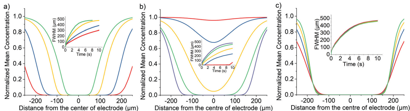
Fig. 3 Simulated optical responses for the mediated oxidation mechanism ( \text{EC}_2 ). Variation of the normalized concentration of species A as a function of distance perpendicular to the electrode. (a) Plot of the variation in the profile at t = 5 s with initial concentration of A, [A]_{\text{bulk}} , equals to 0.25 mM (red), 0.13 mM (blue), 25 \mu\text{M} (yellow) and 2.5 \mu\text{M} (green); [Y]_{\text{bulk}} = 1 mM, D_A = 1 \times 10^{-5} \text{ cm}^2 \text{ s}^{-1} and k_f = 1 \times 10^4 \text{ L mol}^{-1} \text{ s}^{-1} ; Inlay, plot of full-width half minimum of the concentration profile at t = 0 to 10 s. (b) Plot of the variation in the profile at t = 5 s with formation rate constant, k_f , varies from 1 to 1 \times 10^4 \text{ L mol}^{-1} \text{ s}^{-1} . [Y]_{\text{bulk}} = 1 mM, [A]_{\text{bulk}} = 25 \mu\text{M} and D_A = 1 \times 10^{-5} \text{ cm}^2 \text{ s}^{-1} ; inlay, plot of full-width half minimum of the concentration profile at t = 0 to 10 s. (c) Plot of the variation in the profile at t = 5 s with diffusion coefficient of A, D_A , equals to 2 \times 10^{-5} \text{ cm}^2 \text{ s}^{-1} (red), 1 \times 10^{-5} \text{ cm}^2 \text{ s}^{-1} (blue), 6 \times 10^{-6} \text{ cm}^2 \text{ s}^{-1} (yellow) and 3.85 \times 10^{-6} \text{ cm}^2 \text{ s}^{-1} (green); [Y]_{\text{bulk}} = 1 mM, [A]_{\text{bulk}} = 25 \mu\text{M} and k_f = 1 \times 10^4 \text{ L mol}^{-1} \text{ s}^{-1} ; inlay, plot of full-width half minimum of the concentration profile at t = 0 to 10 s. Other parameters: D_Y = D_Z = D_B = 1 \times 10^{-5} \text{ cm}^2 \text{ s}^{-1} , K_{\text{eq}} = 1 \times 10^{10} \text{ M}^{-1} , k_0 = 1 \times 10^4 \text{ cm s}^{-1} .
