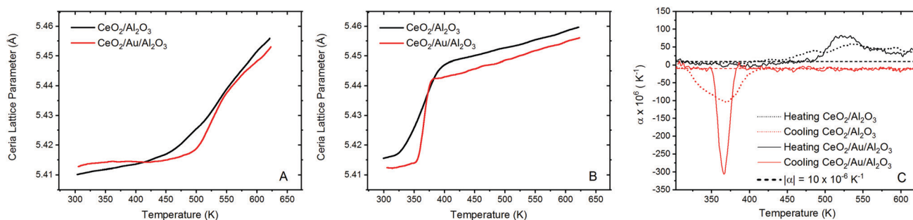
Fig. 3 Experimental DxpPDF results showing the extracted ceria lattice parameter. The ceria/alumina and ceria/Au/alumina ceria lattice parameter refinements are given in black and red respectively for experiments conducted during heating in a 5% H 2 /He atmosphere for the ceria (A) and cooling (B) in 5% H 2 /He (C) instantaneous expansion coefficient during heating and cooling for the ceria/alumina (dotted lines) and ceria/Au/alumina (solid lines) samples. Dashed lines give the expected thermal expansion coefficient of ceria, \alpha = 10 \times 10^{-6} \text{ K}^{-1} , expansion in excess is associated to chemical change of the sample.
