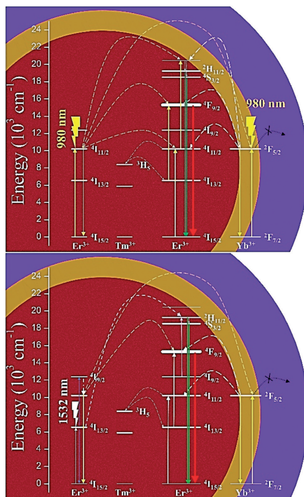
Fig. 6 The proposed energy transfer mechanisms of \beta\text{-NaErF}_4:0.005\text{Tm}@ \text{NaYbF}_4@ \text{NaYF}_4 CSS UCNs excited with 980 nm laser (top) and 1532 nm lasers (bottom), respectively.
