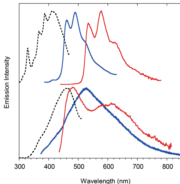
Fig. 2 Emissive behavior of compounds 1 (top) and 3 (bottom) as crystalline powders. PL spectra (blue solid lines; 1 \lambda_{ex} = 330 nm, 3 \lambda_{ex} = 335 nm), PLE spectra (black dashed lines; 1 \lambda_{em} = 490 nm, 3 \lambda_{em} = 525 nm) and phosphorescence spectra (red solid lines; 1 \lambda_{ex} = 410 nm, time delay 1 ms, window 10 ms; 3 \lambda_{ex} = 420 nm, time delay 5 ms, window 15 ms).
