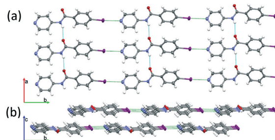
Fig. 3 INPBA structure: (a) 2D sheets formed by N_{\text{pyr}}\cdots\text{I} halogen bonding in green and perpendicular \text{N-H}\cdots\text{O}=\text{C} carboxamide hydrogen bonds in blue; (b) isolated layers. Thermal ellipsoids are drawn at the 50% probability level.
