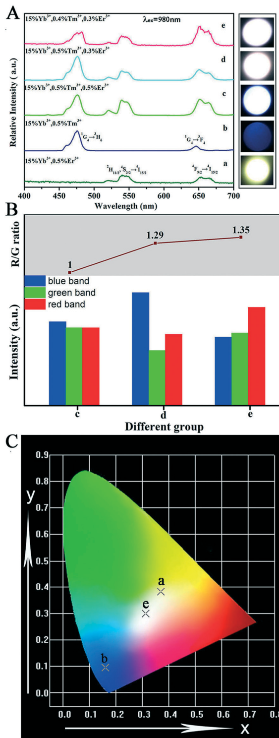
Fig. 11 (A) UC PL spectra of \text{Sr}_2\text{YF}_7:\text{Yb}^{3+}/\text{Er}^{3+}/\text{Tm}^{3+} and their corresponding luminescence photos under 980 nm excitation; (B) intensity ratios of RGB for the group c/d/e A; and (C) CIE chromaticity coordinates of group a/b/e in A.
