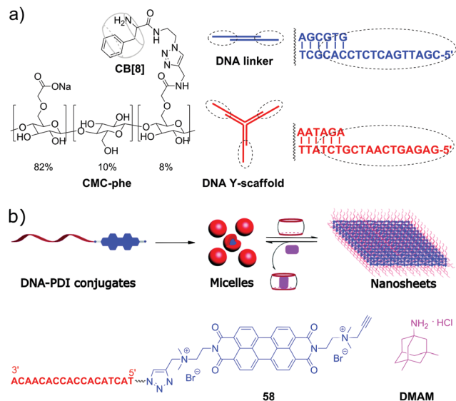
Scheme 13 Formation of supramolecular CB[7]-DNA conjugates and their self-assembly into spherical micelles.
