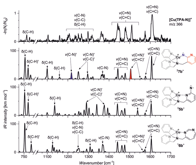
Fig. 3 Helium tagging infrared photodissociation spectrum of [\text{Cu}(\text{TPA-N})]^+ ( m/z 366) (top panel). Theoretical IR spectra of 37b , 35b and 16b were calculated for the optimized structures at the B3LYP/6-31+G* level and scaled by 0.97. \delta(\text{C-H}) , \nu(\text{C=C}) and \nu(\text{C=N}) correspond to the absorption bands in the pyridine rings whereas \delta(\text{C-H})' , \nu(\text{C=C})' and \nu(\text{C=N})' correspond to the absorption bands in the nitrene-pyridine ring.
