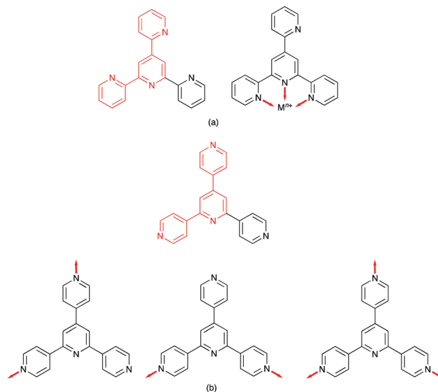
Scheme 2 Examples of tpty motifs as units within quaterpyridines. (a) 4'-(Pyridin-2-yl)-2,2':6',2''-tpty contains a 2,2':4',2''-tpty unit (in red) but typically binds metal ions as a bis(chelate). (b) 4'-(Pyridin-4-yl)-4,2':6',4''-tpty contains a 4,2':4',4''-tpty unit (in red); three possible ditopic modes of bonding of 4'-(pyridin-4-yl)-4,2':6',4''-tpty represented in the CSD by refcode entries AGUPUO (left), QOTREY (middle) and RIGPII (right).
