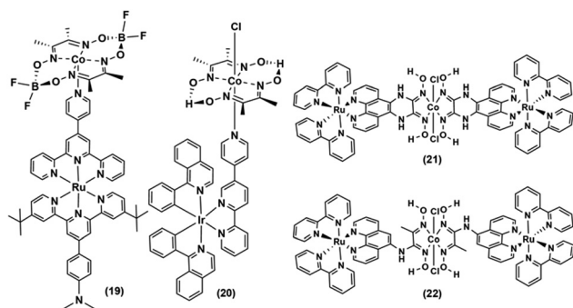
Fig. 4 Various noble metal-based PS-axial- (19–20) and -equatorial-linked (21–22) cobaloximes.
