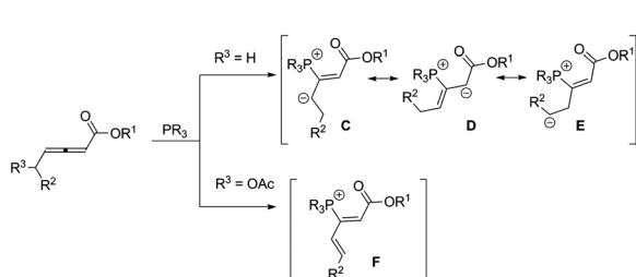
Scheme 1 The reactivity of allenates in the presence of organophosphines.
