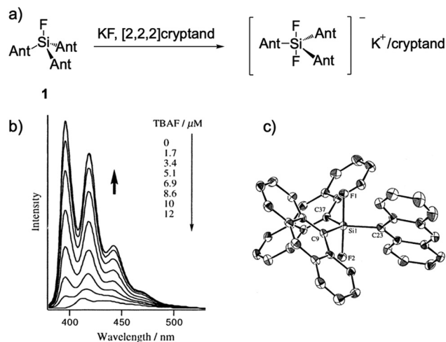
Fig. 1 (a) Reaction scheme of \text{F}^- sensor 1 . (b) Fluorescence titration of 1 with TBAF in THF, [ 1 ] = 0.2 \mu\text{M} . (c) Single crystal structure of the complex, \text{K}^+/\text{[2.2.2]cryptand} is omitted for clarity. Reproduced with permission from ref. 14. Copyright 2000, American Chemical Society.
