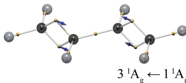
Fig. 5 The electron positions for the mid-point of the vibration, \bar{x} = (\bar{x}_i + \bar{x}_j)/2 , and the displacement vectors x_{fi} for the 1^1B_u \leftarrow 1^1A_g and 3^1A_g \leftarrow 1^1A_g transitions of trans -butadiene. The vector length is doubled for clarity.
