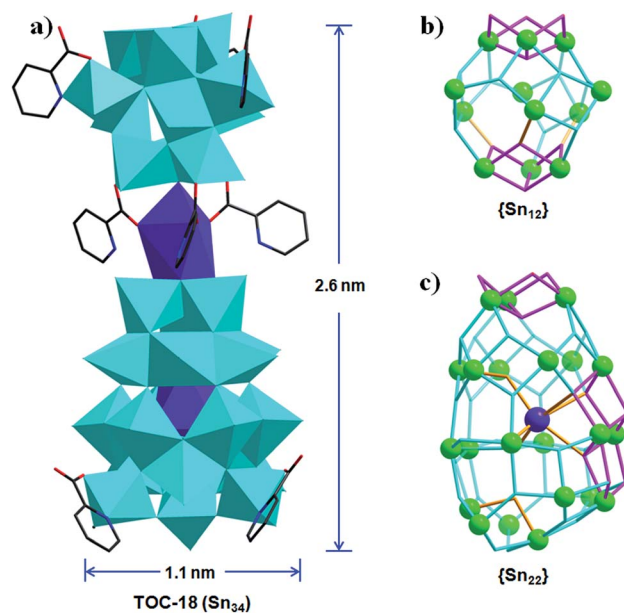
Fig. 3 (a) The polyhedral representation of TOC-18. (b) and (c) The ball-and-stick representations of {Sn 12 } and {Sn 22 } moieties in TOC-18. Polyhedral color code: blue SnO 5 C/SnO 4 C/SnO 4 NC; purple NaO 7 /NaO 6 . Atom color code: green Sn; purple Na; red O; black C; dark blue N.
