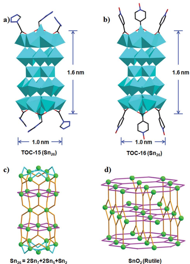
Fig. 2 Polyhedral representations of the Sn 26 cluster in TOC-15 (a) and TOC-16 (b). The ball-and-stick representations of Sn 26 (c) and SnO 2 (rutile) (d). Polyhedral color code: blue SnO 5 C/SnO 3 C/SnO 6 . Atom color code: green Sn.
