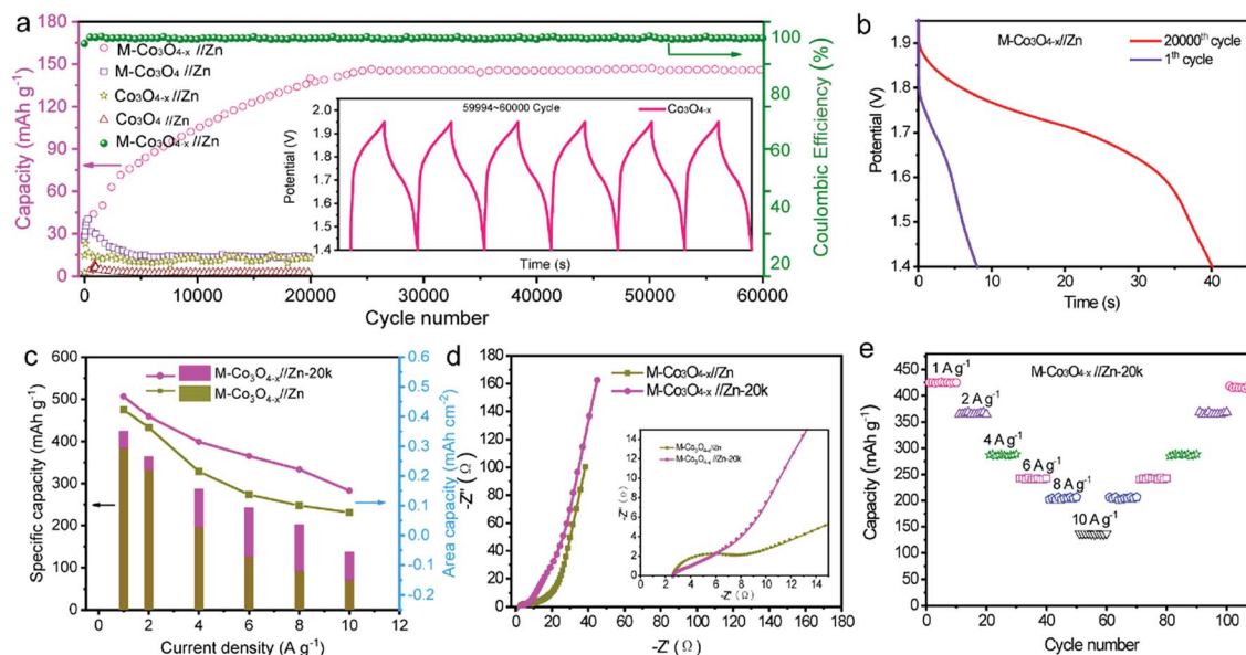
Fig. 5 (a) Cycling performance of M-Co 3 O 4-x /Zn, M-Co 3 O 4 /Zn, Co 3 O 4-x /Zn and Co 3 O 4-x /Zn batteries at 10 A g -1 . (b, c and d) GCD curves, specific capacities at various current densities and Nyquist plots of M-Co 3 O 4-x /Zn and M-Co 3 O 4-x /Zn-20k batteries. (e) Cycling rate performance of M-Co 3 O 4-x /Zn-20k.
