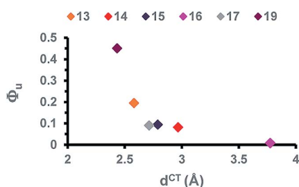
Fig. 4 Correlation between the extent of photo-induced ICT ( d^{\text{CT}} ) and the relative uncaging quantum yields Q_{\text{u}}^{\text{rel}} in compounds 13–17 and 19.
