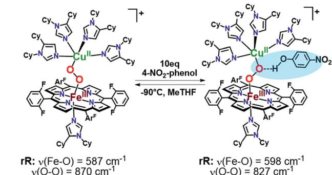
Scheme 2 Previously reported hydrogen-bonding adduct that formed upon addition of 10 equivalents of 4-nitrophenol to a low-spin heme-peroxo-copper complex. Resonance Raman results reported were consistent with the rR in this work (Table 1), where a decrease is observed in the \nu(\text{O-O}) when H-bonding groups interact with the peroxo core.
