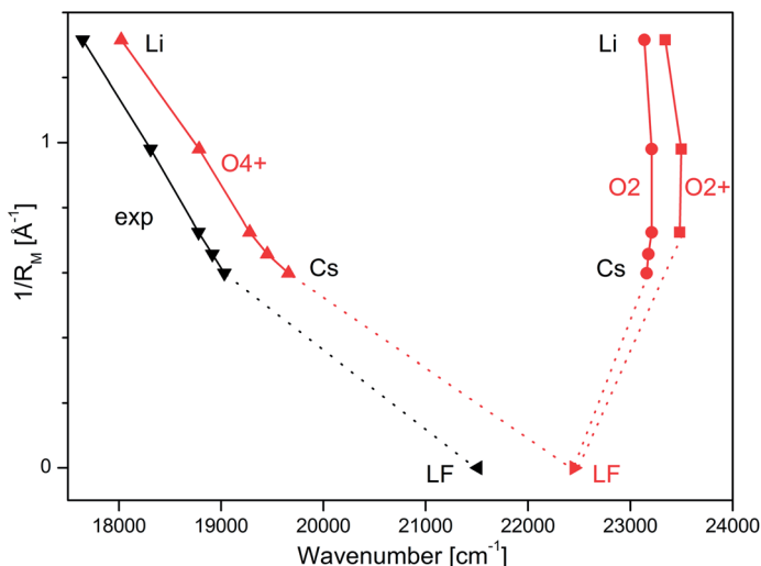
Fig. 3 Experimental S_1 origins extracted from the VSPD spectra of M^+LF compared to adiabatic S_1 origin energies of the O4+ and O2(+) isomers of M^+LF calculated at the PBE0/cc-pVDZ level plotted as a function of the inverse ionic radius of the metal ion ( 1/R_M ). The M^+LF ions with M = Rb and Cs do not have a stable O2+ structure. The experimental value for LF is taken from the He droplet spectrum. 33
