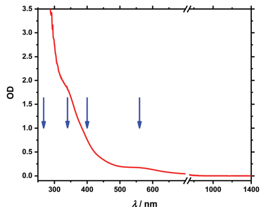
Fig. 2 Stationary absorption spectrum of \text{Fe(CO)}_2\text{CpGe}_9\text{Hyp}_3 between 250 and 1400 nm. Blue arrows mark excitation wavelengths at 258/267, 340, 388/400 and 560 nm, respectively.
