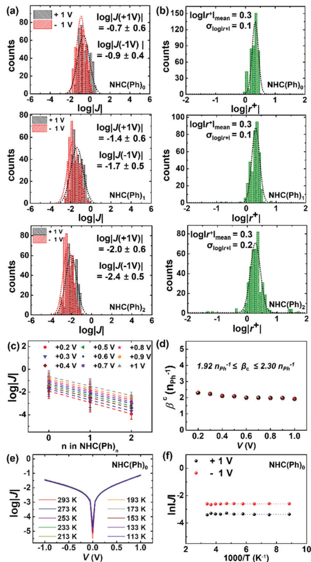
Fig. 2 Histograms of (a) \log|J| and (b) \log|r^+| at \pm 1.0 V for NHC(Ph) _n ( n = 0, 1 , and 2 ) SAM. (c) Linear correlation between the \log|J| and the molecular length. (d) Constant \beta^c value regardless of applied voltage. (e) Exemplary \log|J| – V traces measured at low temperatures (from 113 to 293 K) for Au TS /NHC(Ph) _0 /Ga _2 O _3 /EGaIn junctions. (f) The corresponding Arrhenius plots.
