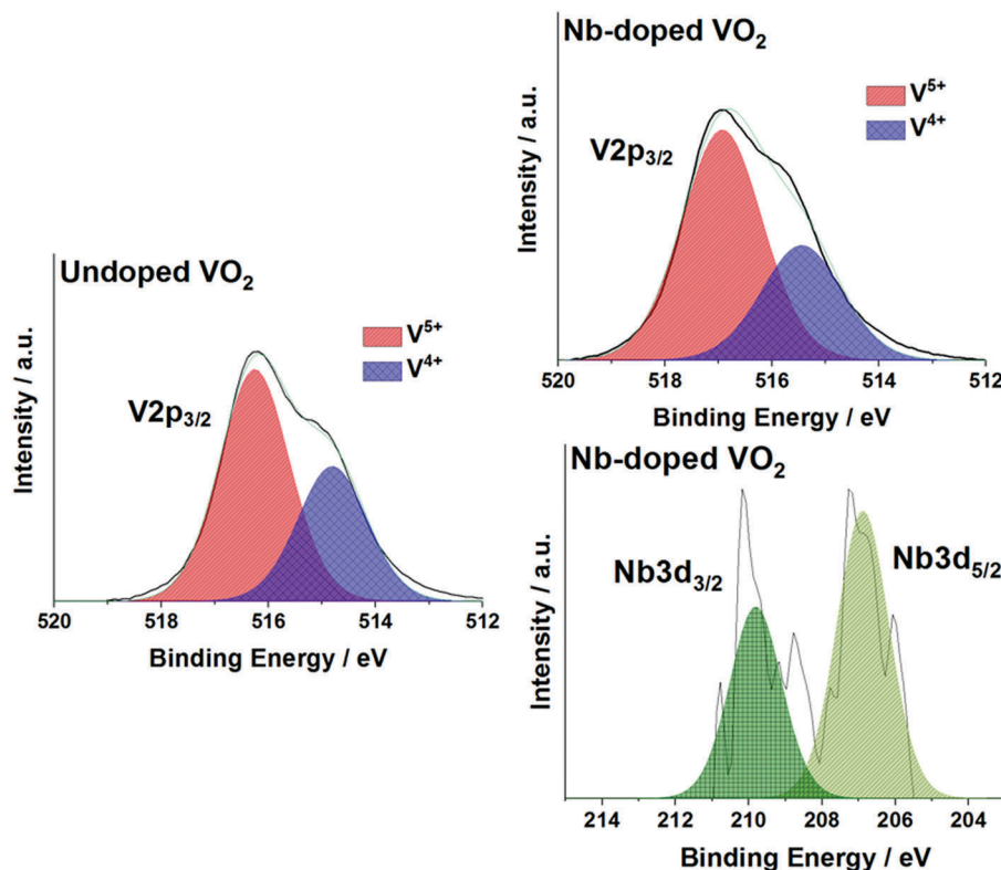
Fig. 5 X-ray photoelectron spectra (XPS) of the V 2p 3/2 and Nb 3d 5/2 environments in the (a) undoped VO 2 and (b) Nb-VO 2 samples.
