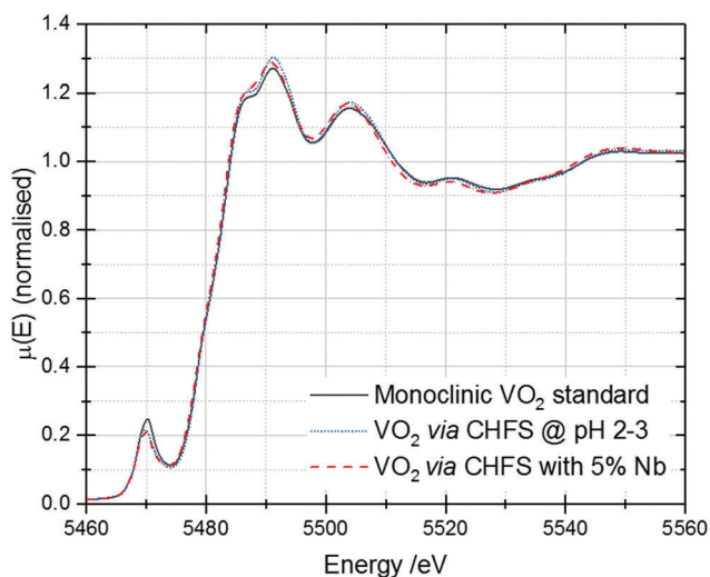
Fig. 6 V K-edge XANES of the VO 2 and Nb-VO 2 samples synthesised by CHFS. A spectrum of a commercial monoclinic VO 2 standard has been included for reference.
