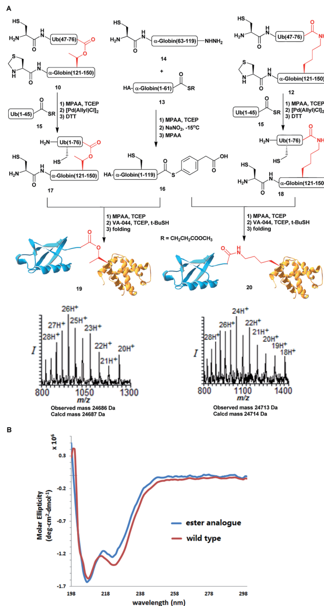
Scheme 3 (A) Syntheses of HA- \alpha -globin-Ub having the ester or isopeptide linkages with the observed masses of 24 686 Da (calcd 24 687 Da) and 24 713 Da (calcd 24 714 Da), respectively. (B) CD analysis of the HA- \alpha -globin-Ub analogues.
