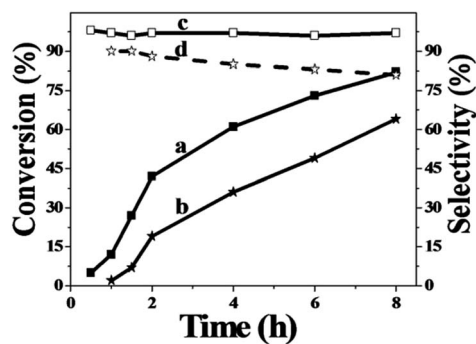
Fig. 3 Dependence of cyclohexene conversion and 2-cyclohexene-1-one selectivity on the reaction time over Au/Zn-MOF catalysts at the reaction conditions of Table 1. (a and c) Conversion and selectivity with 0.8 nm Au particles and (b and d) conversion and selectivity with 1.5 nm Au particles.
