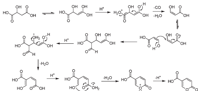
Scheme 2 Postulated mechanism for the synthesis of coumalic acid.
