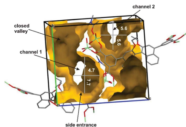
Fig. 2 Connolly's surface calculated from X-ray structure of ( R )-ZnMOF-4 showing diameters and topology of two channels.
