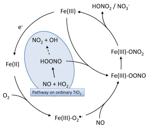
Fig. 11 The proposed reaction mechanisms for peroxyntrite/peroxyntinous acid isomerization on the grafted Fe(III) that would prevent NO 2 release through peroxyntinous acid decomposition.
