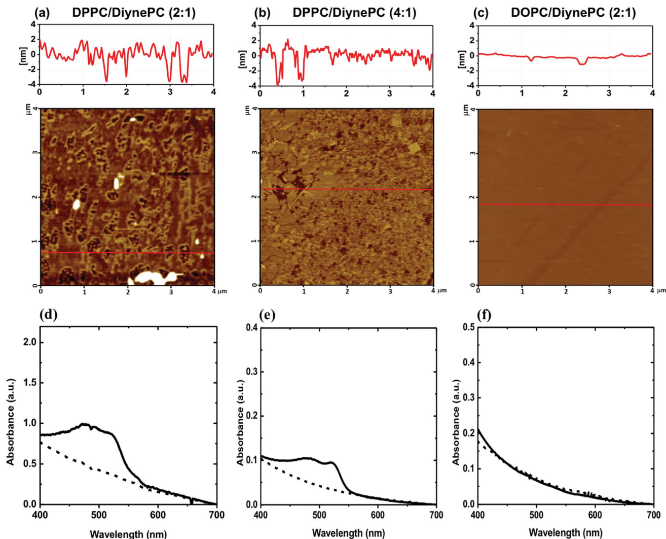
Fig. 5 (a–c) AFM images of lipid bilayers containing DiynPC after photo-polymerization (254 nm, 2 \text{ mW cm}^{-2} , 15 min) in liquid environment. Pore size of (a) is 191 \pm 128 \text{ nm} , (b) is 122 \pm 70 \text{ nm} and (c) is not found. (d and e) Visible absorption spectra before (dashed line) and after (solid line) polymerization of vesicles; (a and d) DPPC/DiynPC (2 : 1), (b and e) DPPC/DiynPC (4 : 1) and (c and f) DOPC/DiynPC (2 : 1) mixtures.
