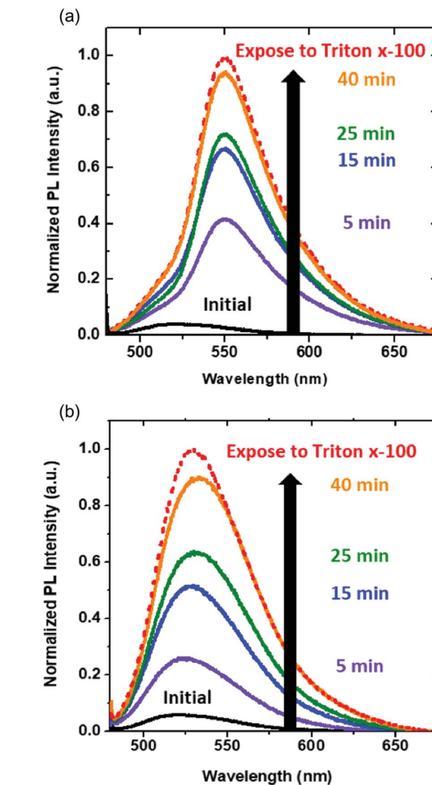
Fig. 6 Effect of composition of DiynPC on calcein release from vesicles by exposure to UV light with time. Triton X-100 line means 100% calcein release; (a) DPPC/DiynPC (2 : 1) vesicles and (b) DPPC/DiynPC (4 : 1) vesicles.
