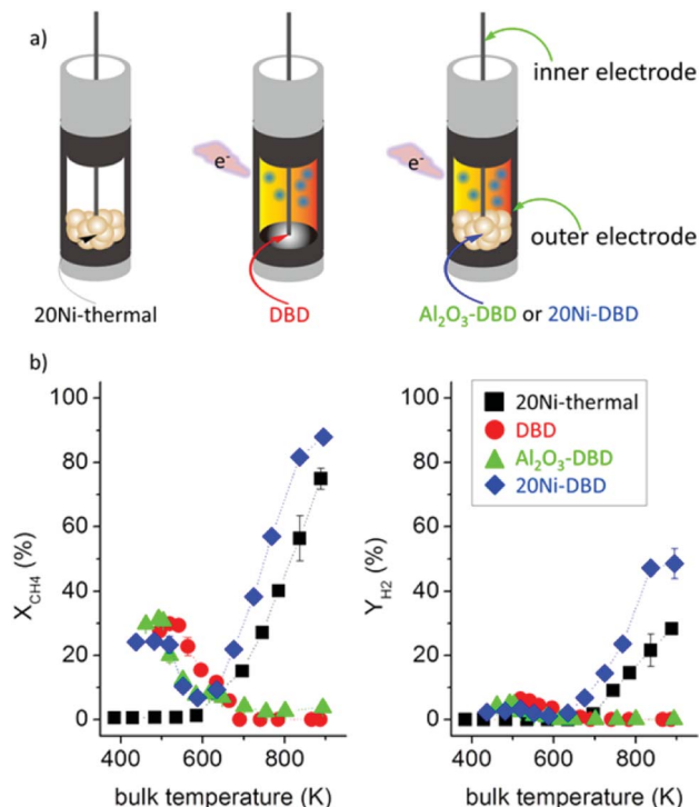
Fig. 6 (a) Reaction environments for the CH 4 reforming and (b) profiles of CH 4 conversions ( X_{\text{CH}_4} ) and H 2 yields ( X_{\text{H}_2} ) at various reaction environments obtained via bulk temperature controls. Reproduced from ref. 200 with permission from American Chemical Society, copyright 2016.
