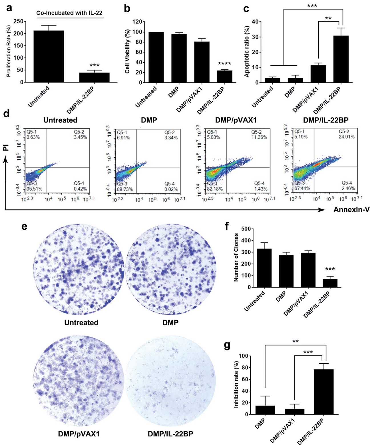
Fig. 3 DMP/IL-22BP complex efficiently inhibit the growth of C26 cancer cells in vitro . (a) expressing of IL-22BP blocked IL-22-based cell proliferation signal; (b) inhibition effect of DMP/IL-22BP complex detected by MTT assay; (c) and (d) DMP/IL-22BP complex efficiently induced apoptosis in C26 cells; (e) inhibition effect of DMP/IL-22BP complex evaluated by clonogenic assay, the numbers of clones in each well were counted (f) and translated into inhibition rate (g).
