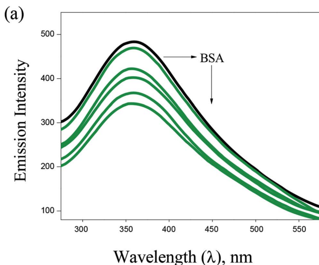
Fig. 7 Fluorescence spectra of BSA (10 \mu M, \lambda_{\text{ex}} = 280 nm, \lambda_{\text{em}} = 570 nm) in the presence of increasing concentrations of 2 (a) and 3 (b). Arrow shows that the emission intensity changes upon increasing the concentration of the complexes.
