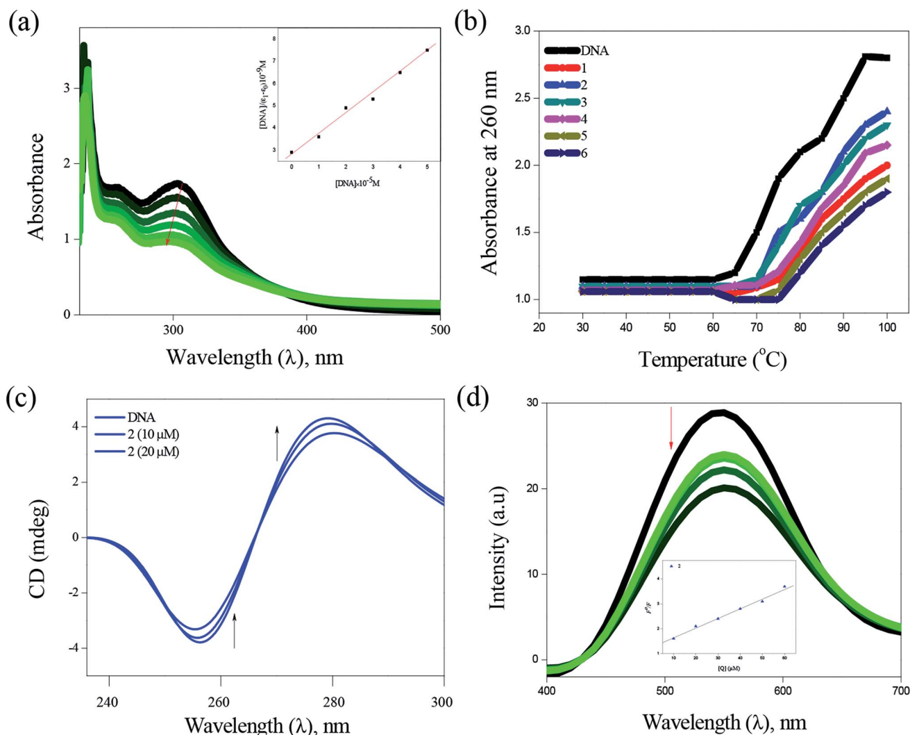
Fig. 4 DNA binding of complexes with CT-DNA: absorption spectra of complex 2 (a), thermal denaturation of complexes 1–6 (b), CD spectra of complex 2 (c) and emission spectra of complex 2 (d).
