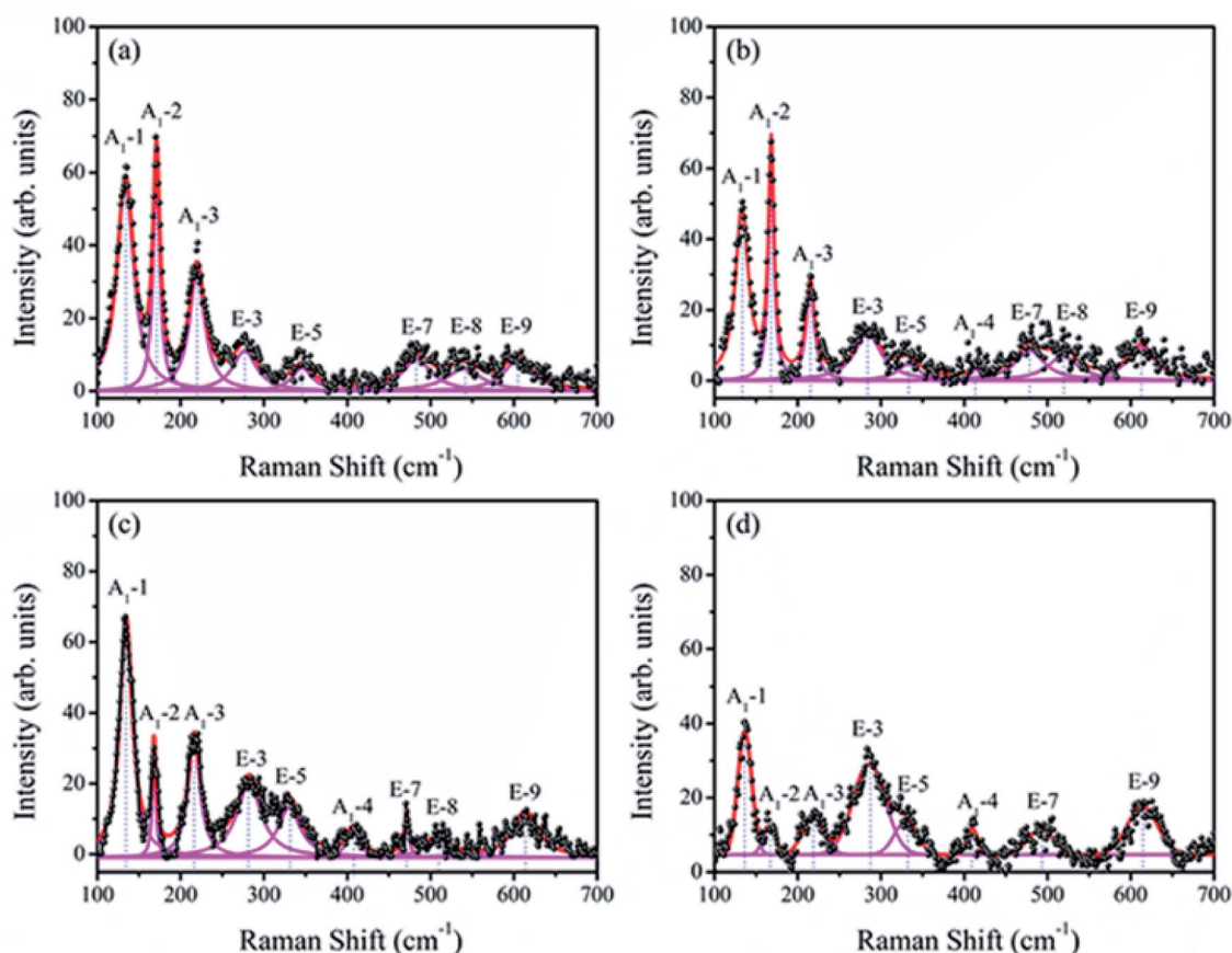
Fig. 4 Raman scattering spectra of \text{BiFeO}_3 (a), \text{Bi}_{98.59\%}\text{La}_{0.67\%}\text{Pr}_{0.74\%}\text{FeO}_3 (b), \text{Bi}_{97.80\%}\text{La}_{0.61\%}\text{Pr}_{1.59\%}\text{FeO}_3 (c) and \text{Bi}_{96.35\%}\text{La}_{0.94\%}\text{Pr}_{2.71\%}\text{FeO}_3 (d) powders.
