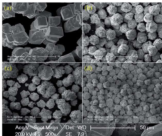
Fig. 2 SEM morphology images of the \text{Bi}_{1-x-y}\text{La}_x\text{Pr}_z\text{FeO}_3 ( x = 0 and 0.05 ; y = 0 (a), 0.10 (b), 0.15 (c) and 0.20 (d)) powders.
