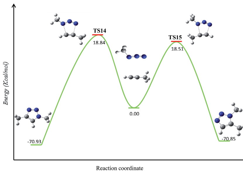
Fig. 4 Calculated energy (kcal mol -1 ) barriers for the uncatalyzed thermal azide-alkyne 32CA reaction in absence of copper(I) species.
