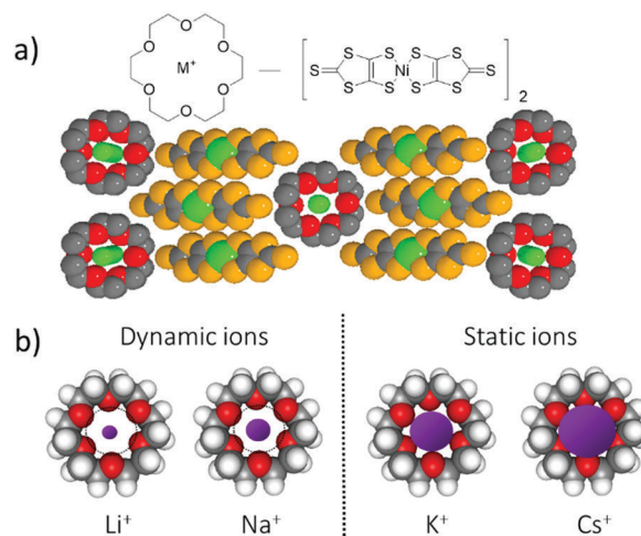
Fig. 8 Dynamic ( \text{M}^+ = \text{Li}^+ and \text{Na}^+ ) and static ( \text{M}^+ = \text{K}^+ and \text{Cs}^+ ) ionic channels in conducting \text{M}^+ \cdot [\text{18}]\text{crown-6}[\text{Ni}(\text{dmit})_2]_2 salts. (a) Molecular structures and packing structure. The motional freedom of the cations affected the potential for the conduction electrons on the \pi -stack of partially oxidized [\text{Ni}(\text{dmit})_2] . (b) Dynamic and static ion environments were observed according to the size of the alkali metal ions ( \text{Li}^+ , \text{Na}^+ , \text{K}^+ , and \text{Cs}^+ ) and cavity size of the [18]crown-6 ether.
