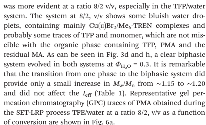
SET-LRP of MA catalyzed by non-activated Cu(0) wire/TREN/ Cu(II)Br 2 in TFE/water and TFP/water mixtures
