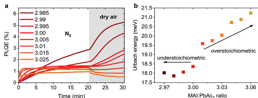
Fig. 5 (a) Evolution of the photoluminescence quantum efficiency (PLQE) under different atmospheres (0–20 min: N 2 , 20–30 min: dry air) measured with a 440 nm CW laser (~80 mW cm −2 ) inside an integrating sphere flushed with the corresponding gas. (b) Urbach energy determined by photothermal deflection spectroscopy (PDS).
