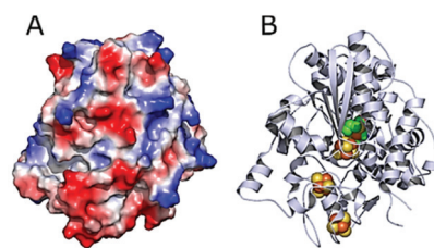
Fig. 5 Structure of DdHdAB (PDB 1HFE). 44 (A) Surface vacuum electrostatic potential distribution of DdHdAB showing negative regions (red) and positive regions (blue) (calculated with PyMol). (B) 3D structure of DdHdAB showing the deeply buried active site (green/yellow), the iron-sulfur clusters (orange/yellow) and the protein shell (gray).
