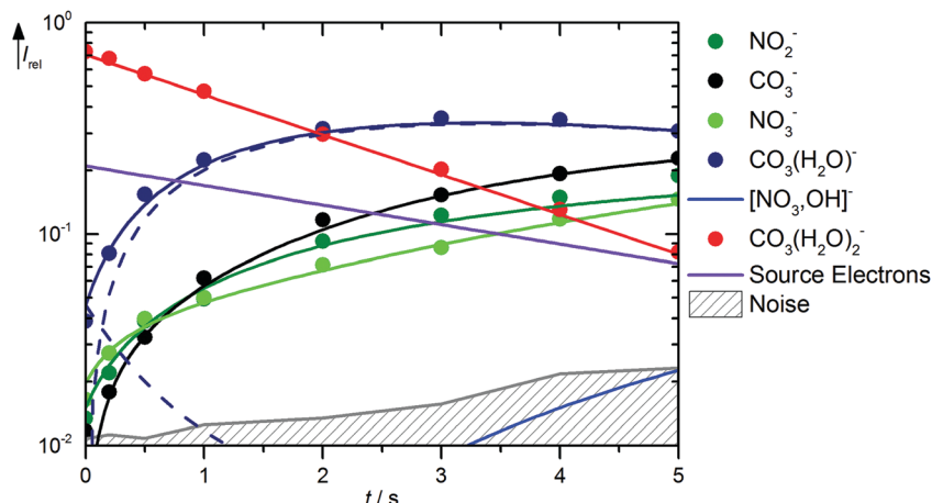
Fig. 4 Kinetics of the reaction of \text{CO}_3^{2-}(\text{H}_2\text{O})_2 with \text{HNO}_3 and \text{H}_2\text{O} , with traces of \text{HONO} , at a \text{HNO}_3 partial pressure of 8.1 \times 10^{-9} mbar. The lines represent the fit with the rate coefficients from Table S3 (ESI†). Selected mass spectra are shown in Fig. S7 (ESI†).
