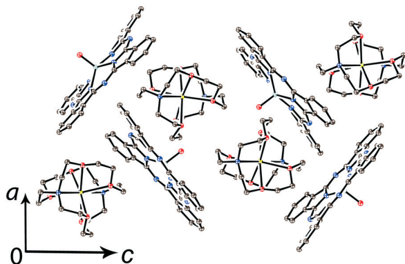
Fig. 6 View of the crystal structure of \{\text{cryptand}(\text{Na}^+)\{\text{V}^{\text{IV}}\text{O}(\text{Pc}^{3-})\}^- \cdot \text{C}_6\text{H}_4\text{Cl}_2 (15) along the b axis and channels occupied by solvent \text{C}_6\text{H}_4\text{Cl}_2 molecules (not shown for clarity) and the cryptand( \text{Na}^+ ) cations. 27
