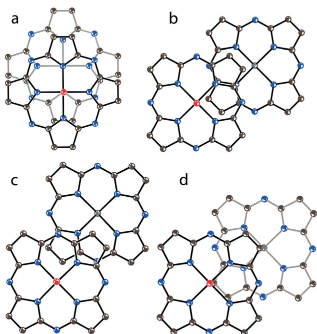
Fig. 12 View of the \pi -stacking \{Ti^{IV}(O(Pc^{3-}))_2\}^- dimers along the M=O bonds: (a) optimal overlapping observed in 1 , 8 and 13 ; (b) partial overlapping observed in 2 ; (c) weak overlapping observed in 4 and 9 ; (d) intermediate overlapping in 12 . Only 24-atom Pc planes are shown.
