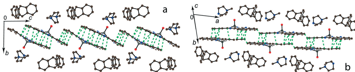
Fig. 11 View along the phthalocyanine layers composed of the \{Ti^{IV}(O(Pc^{3-}))_2\}^- dimers in 12 : view along the a (a) and approximately along the c (b) axes. Short van der Waals contacts between phthalocyanines are shown by green dashed lines.
