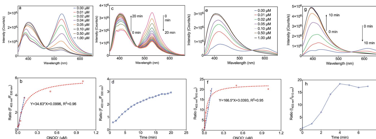
Fig. 3 Properties of the MA and MB sensors. Excitation: 340 nm. (a) Fluorescence spectra of MA ( 1\text{ mg L}^{-1} ) upon addition of various amounts of \text{ONOO}^- (from 0.00 to 1.00\text{ }\mu\text{M} ) in PBS buffer solution (pH 7.4) for 30 min; (b) non-linear correlation between the emission intensity ratio ( F_{403\text{ nm}}/F_{530\text{ nm}} ) and the concentration of \text{ONOO}^- ; (c) fluorescence spectra of MA ( 1\text{ mg L}^{-1} ) with the addition of 1.00\text{ }\mu\text{M} \text{ONOO}^- over time (0 to 20 min); (d) non-linear correlation between the emission intensity ratio ( F_{403\text{ nm}}/F_{530\text{ nm}} ) and time; (e) fluorescence spectra of MB ( 1\text{ mg L}^{-1} ) upon addition of various amounts of \text{ONOO}^- (from 0.00 to 1.00\text{ }\mu\text{M} ) in PBS buffer solution (pH 7.4) for 30 min; (f) non-linear correlation between the emission intensity ratio ( F_{403\text{ nm}}/F_{610\text{ nm}} ) and the concentration of \text{ONOO}^- ; (g) fluorescence spectra of MB ( 1\text{ mg L}^{-1} ) with the addition of 1.00\text{ }\mu\text{M} \text{ONOO}^- over time (0 to 10 min); (h) non-linear correlation between the emission intensity ratio ( F_{403\text{ nm}}/F_{610\text{ nm}} ) and time.
